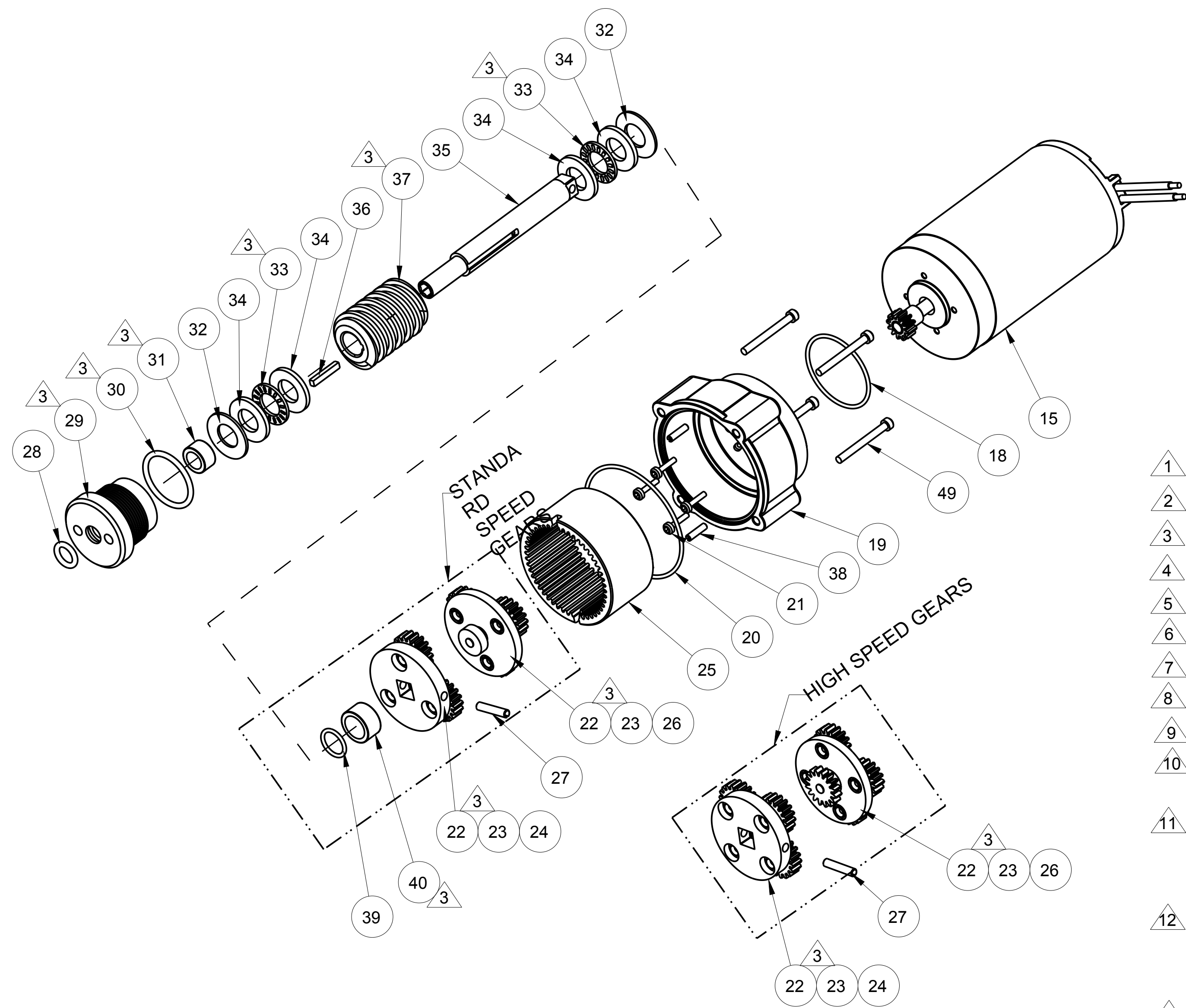
MOTOR/GEARBOX ASSEMBLY FOR BOTH ELEVATION AND ROTATION JOINTS
